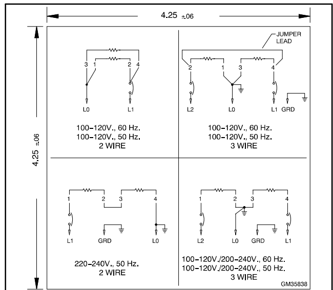
Figure 3 Correct Reconnection Decal (GM35838) for EOZD/EFOZD Units with ADC 2100
