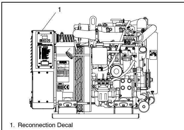
Figure 1 Reconnection Decal Location
