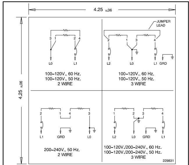
Figure 2 Incorrect Reconnection Decal (229831) for EOZD/EFOZD Units with ADC 2100
